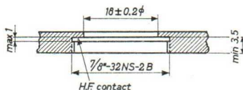
Fig. 2 Recommended mount
