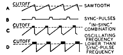
Fig. 102—Sawtooth and sync pulses in synchroguide circuit.
