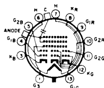
13C Anode = G_4 + CL Focusing Electrode = G_3
