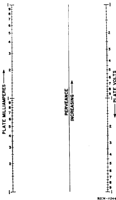
Fig. 125—Diode perveance nomograph.
