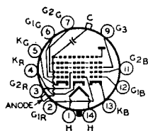
14AU Anode = G_4 + G_5 + CL Focusing Electrode = G_3
