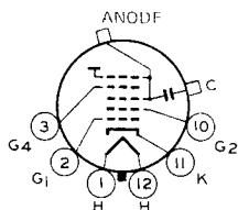
12AB Anode = G_2 + G_3 + CL Focusing Electrode = G_4
