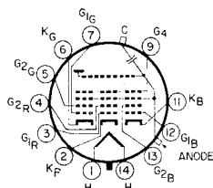
14BH Anode = G_3 + G_5 + CL Focusing Electrode = G_4
