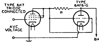
Fig. 111—Indicating circuit using 6AF6G electron-ray tube and external dc amplifier.
