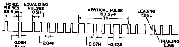
Fig. 81—Waveform of TV synchronizing pulses ( H = horizontal line period of 1/15,750 seconds, or 63.5 \mu s ).
