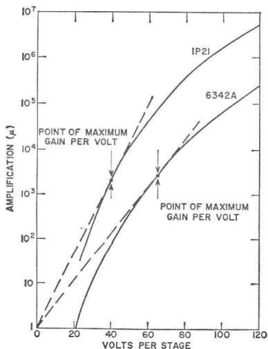
Fig. 36. Log of gain as a function of volts per stage for a tube (IP21) with Cs-Sb dynodes and for a tube (6342A) with Cu-Be dynodes.
