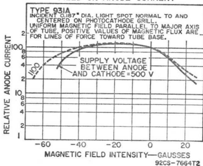
TYPICAL EFFECT OF MAGNETIC FIELD ON ANODE CURRENT
