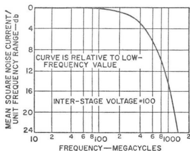
Fig. 56. Power spectrum of the noise from the RCA 931 multiplier phototube operated at 100 volts per stage, as calculated by R. D. Sard.
