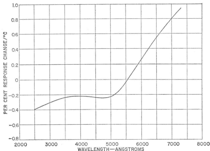
Fig. 43. Temperature coefficient of Cs-Sb cathodes as a function of wavelength; data taken at 20 degrees centigrade. Note the large positive effect near the threshold.
