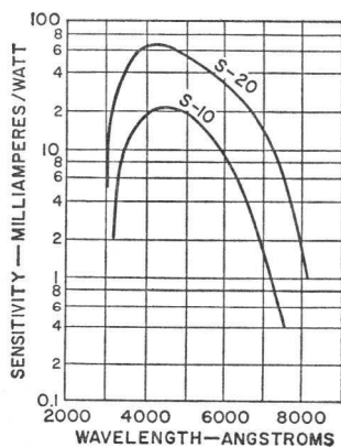
Fig. 39. Spectral response characteristics for S-10 (Bi-Ag-O-Cs photocathode) and S-20 ( [Cs]Na_2KSb photocathode).
