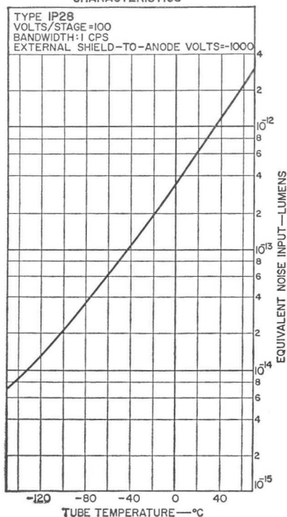
EQUIVALENT-NOISE-INPUT CHARACTERISTICS
