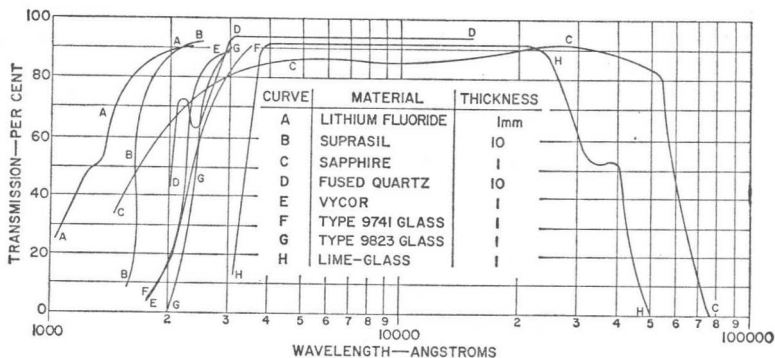
Fig. 19. Transmission characteristics of various glasses used in phototube manufacture.
