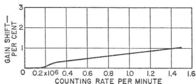
Fig. 69. Typical variation of pulse height with pulse-count rate for a 6342A. ( \text{Cs}^{137} source with a NaI (Tl) source).
