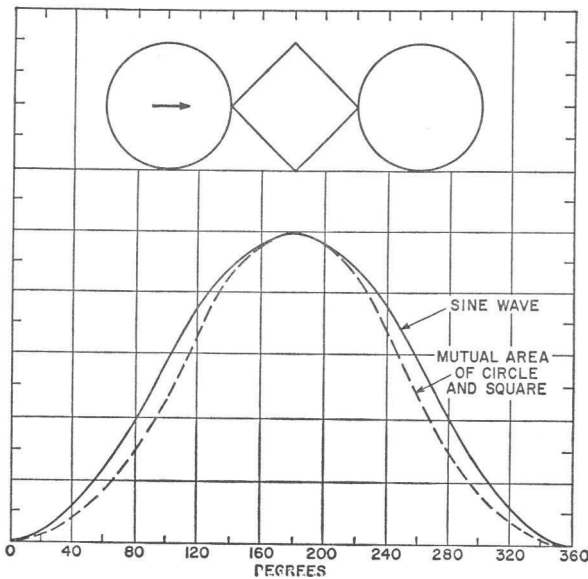
Fig. 92b. Production of sine-wave approximation by use of circular holes and a square aperture of 45 degrees.
