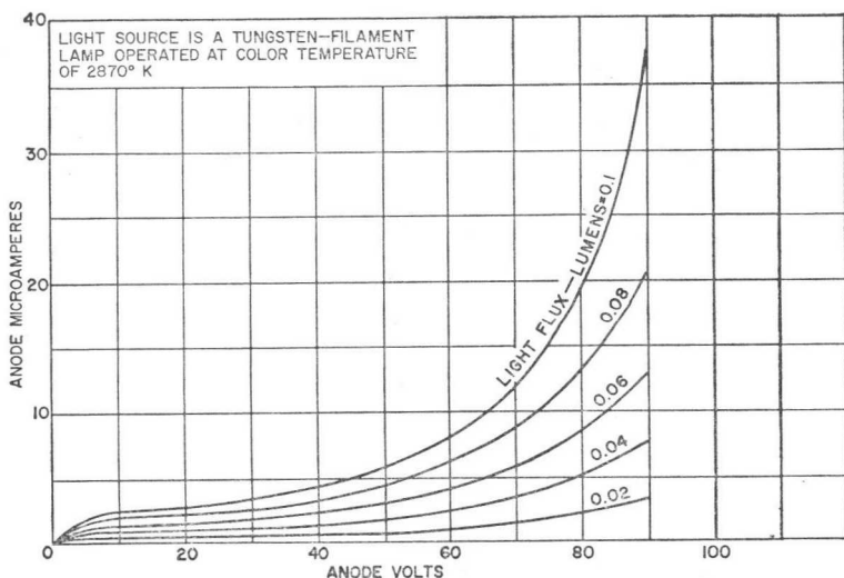
Fig. 26. Current-voltage characteristics for various light levels for a type 918 gas-filled phototube. Some nonlinearity with light is observed at maximum currents.
