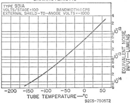
EQUIVALENT-NOISE-INPUT CHARACTERISTIC
