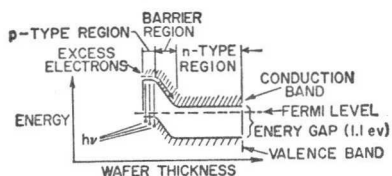
Fig. 9. Energy model of a silicon solar cell.
