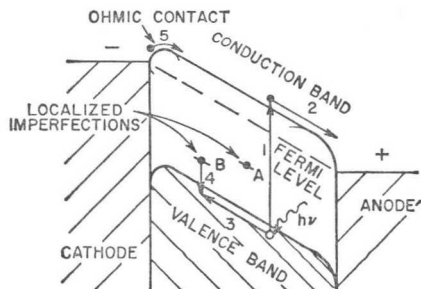
Fig. 8. An n-type photoconductor in operation. Two ohmic metallic contacts to the photoconductor are assumed.
