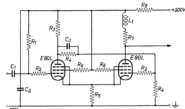
Fig. 28. Additional input pulse shaper for the circuit of Fig. 27.
