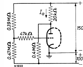
Fig. 31. Circuit in which I_a = \begin{cases} \text{minimum } 5.1 \text{ mA} \\ \text{maximum } 5.9 \text{ mA} \end{cases}
