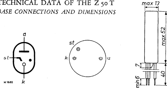
Fig. 48. Electrode arrangement, electrode connections and maximum dimensions in mm.
