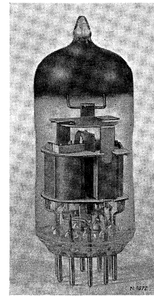
Fig. 35. The E 88 CC (actual size).
