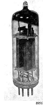
Fig 15. Photograph of the E 90 CC (actual size).
