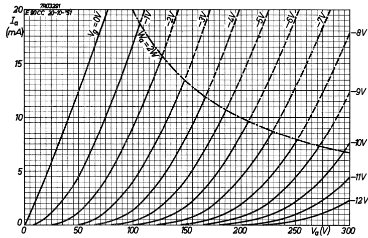
Fig. 19. Anode current I_a of the E 90 CC as a function of the anode voltage V_a with the grid voltage V_{g1} as parameter.
