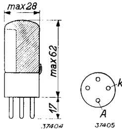
Electrode connections, and maximum dimensions in millimetres.
