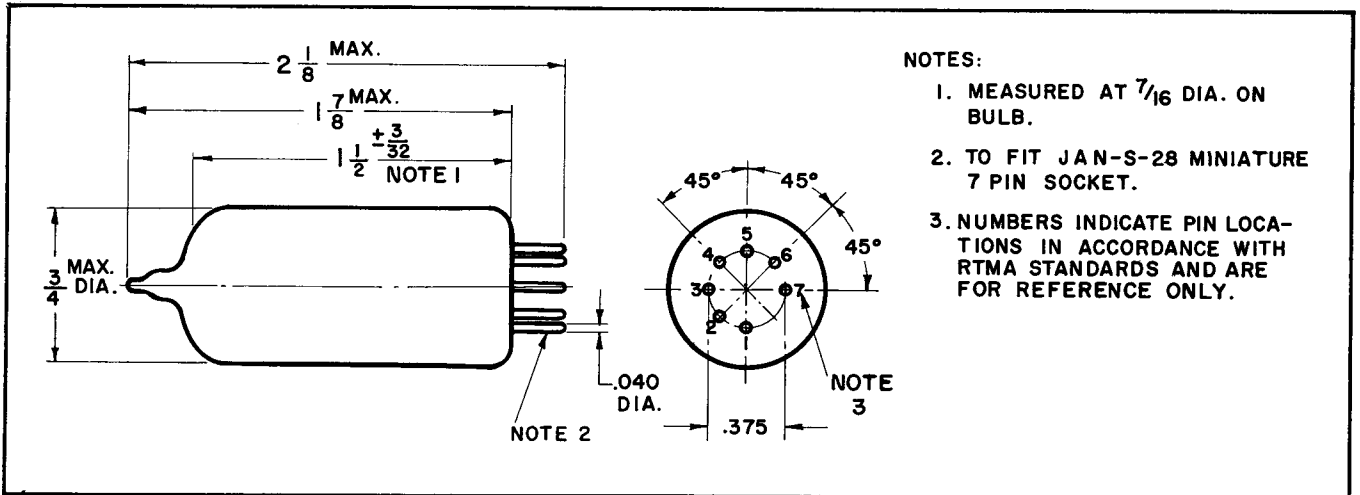
OUTLINE DRAWING
