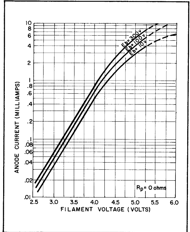
AVERAGE EMISSION CHARACTERISTICS
