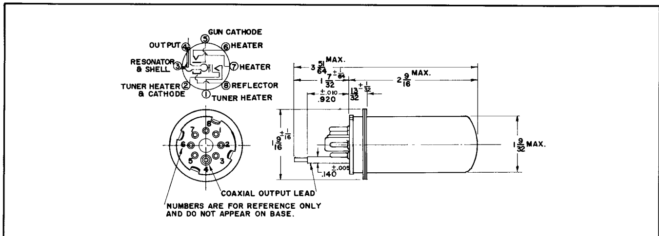
OUTLINE DRAWING
